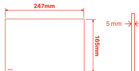
The dimensions of all flush plates
